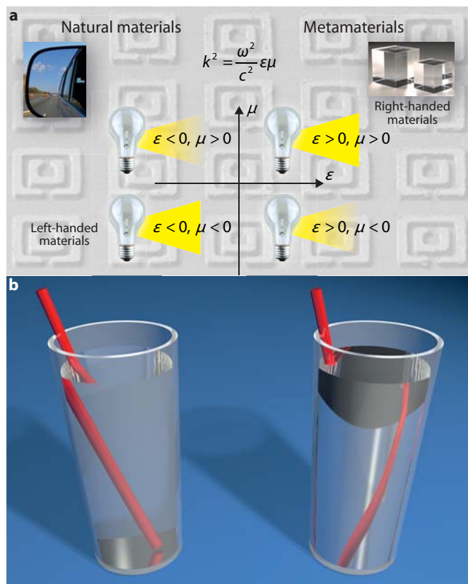
Figure 1. (a) The regions of possible permittivity ( \epsilon ) and permeability ( \mu ), showing normal refraction (top right) and negative refraction (bottom left). (b) Normal refraction (left) and left-handed refraction (right).
